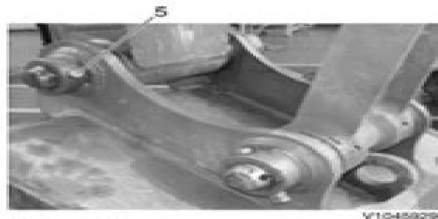
Figure 2075 Bucket pin lock screw, installation
