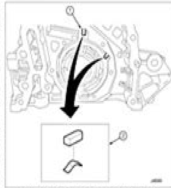
10.10k Fit the new oil pump side oil and side oil spring into the side of the valve cover.
