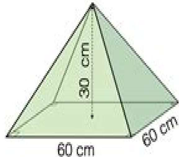
Square-based pyramid
