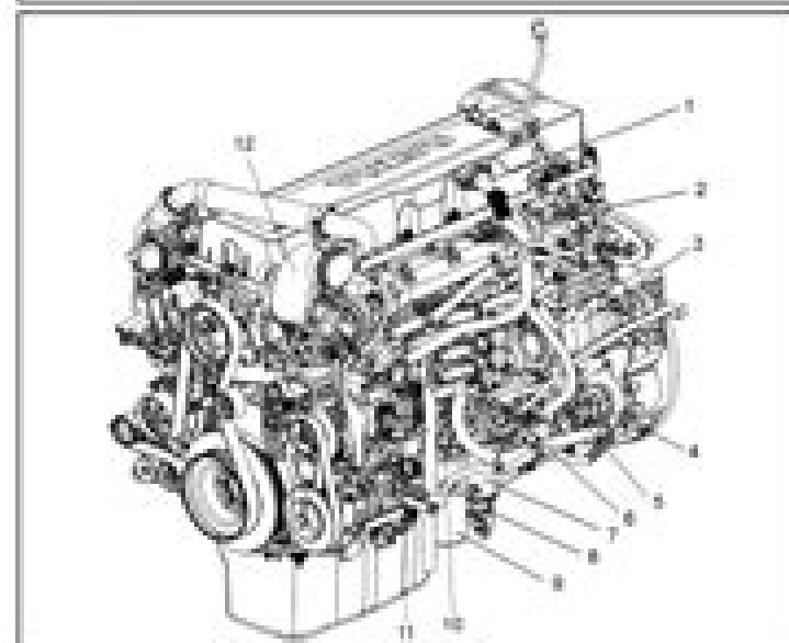
Figure 1. Front view, 4-cylinder Volvo D13 (1200kW)
