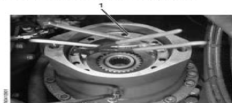
Figure 365 Brake piston 1 Brake piston
