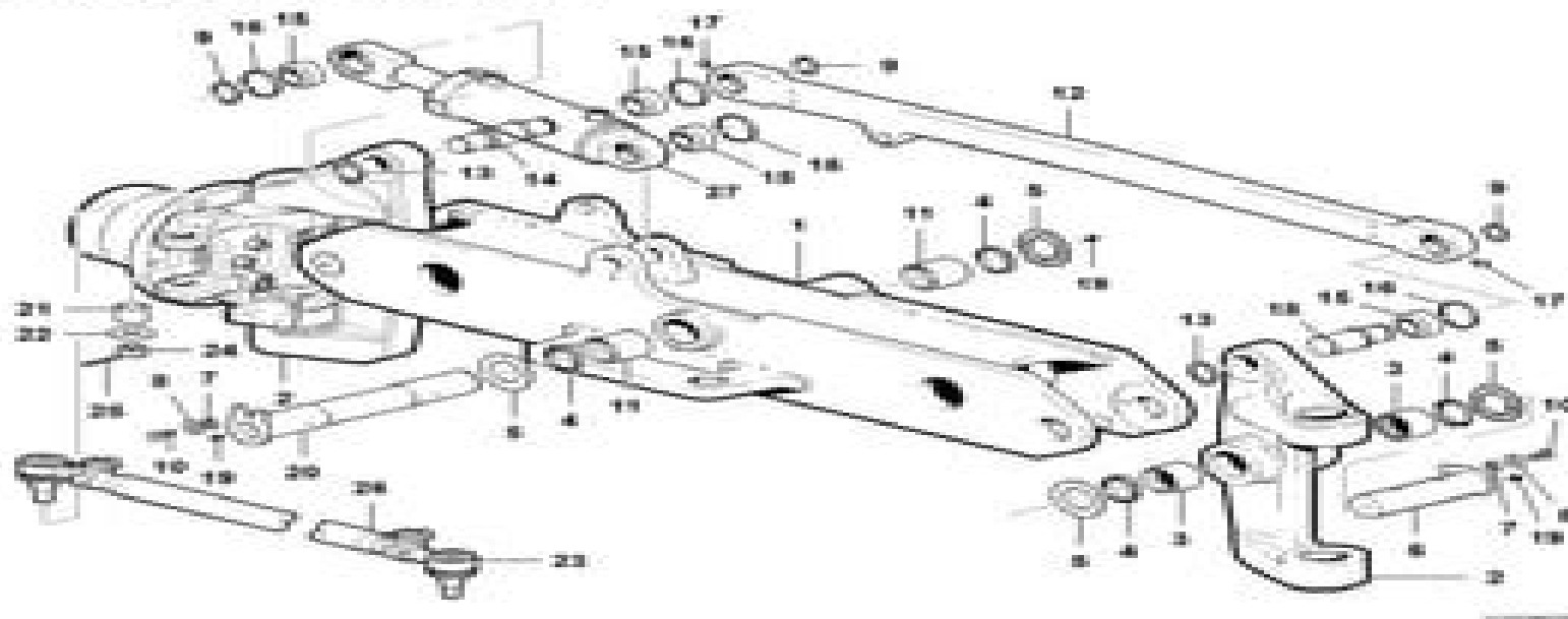
Figure 1 Front axle assembly — G540, G540 G5R and G540
