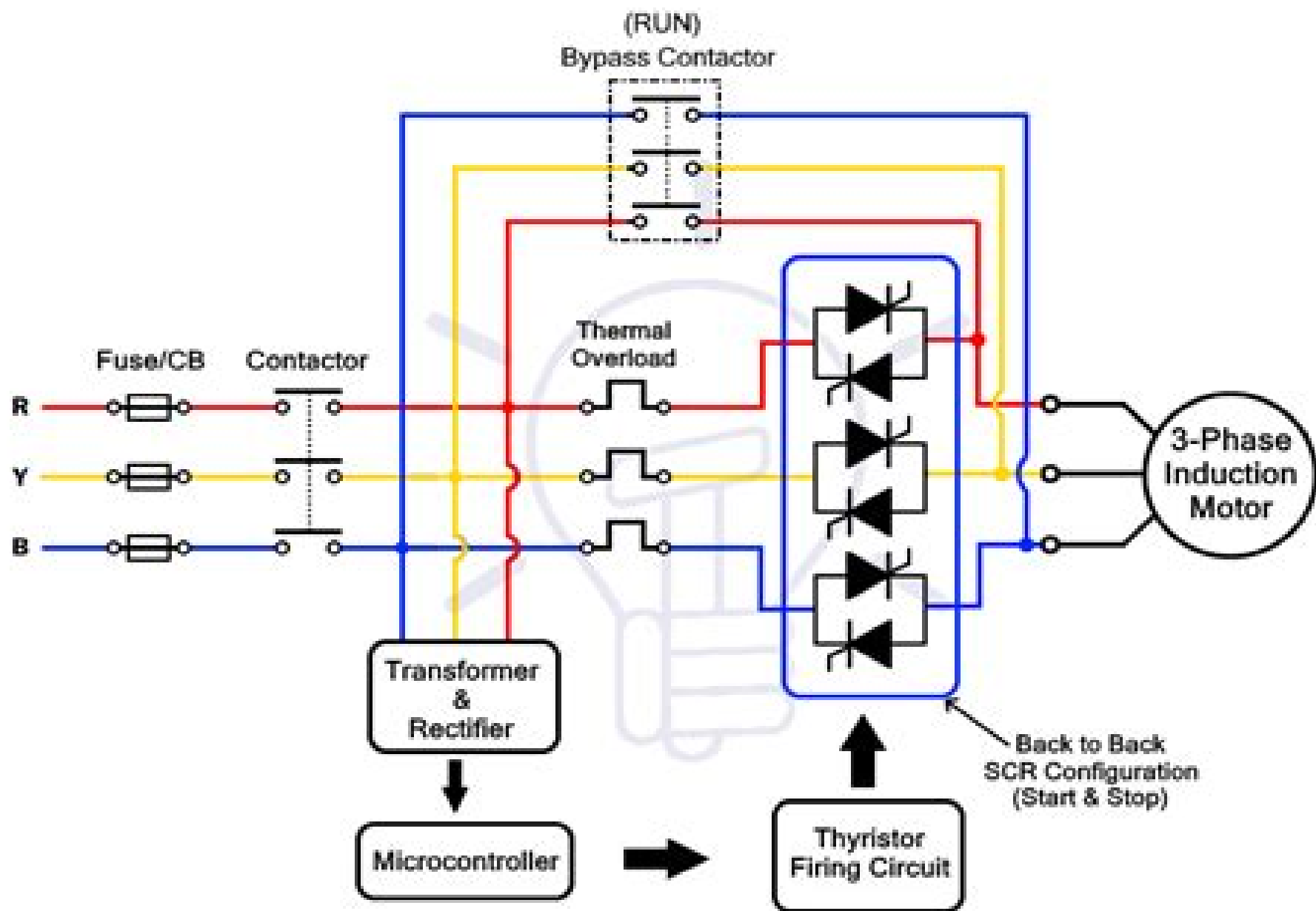
Soft Starter
