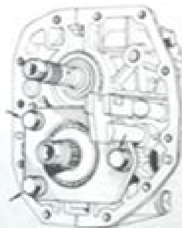
Fig. 6.27 Retorque the bearing cap plate onto the rear face of the 369 gearbox (See 6)
