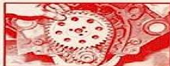
FIGURE 2a. Removing timing gear and chain.
