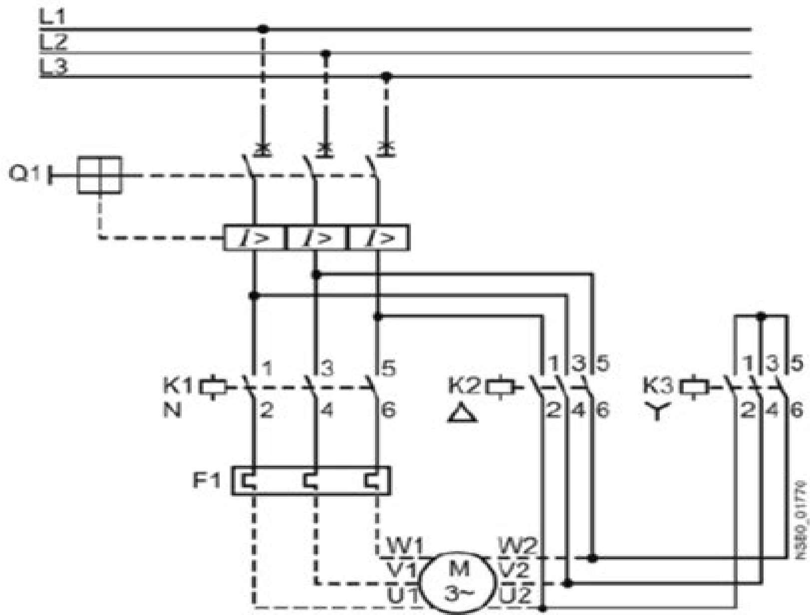
Circuit diagram main circuit for YΔ circuit
