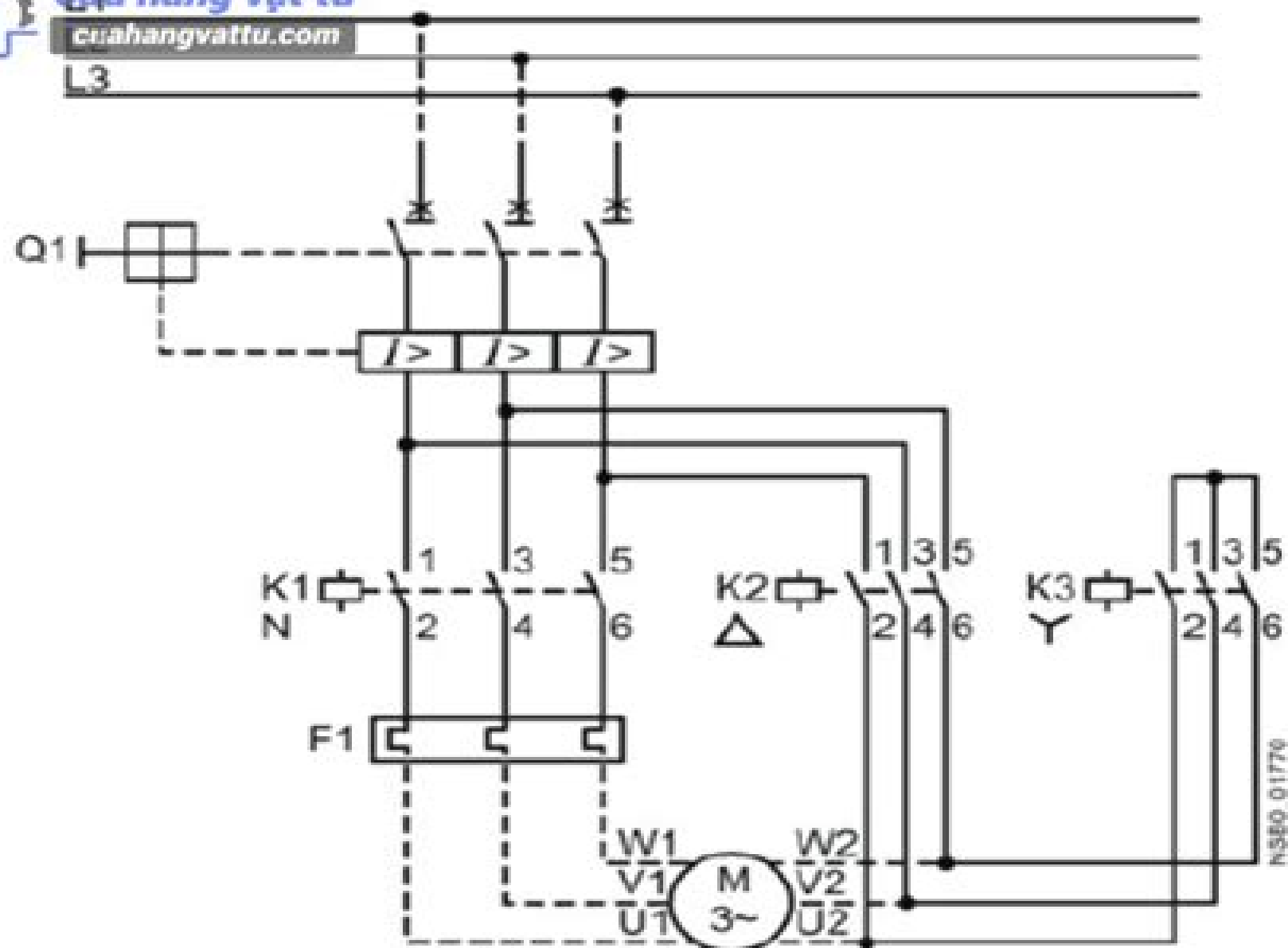
Circuit diagram main circuit for YΔ circuit
