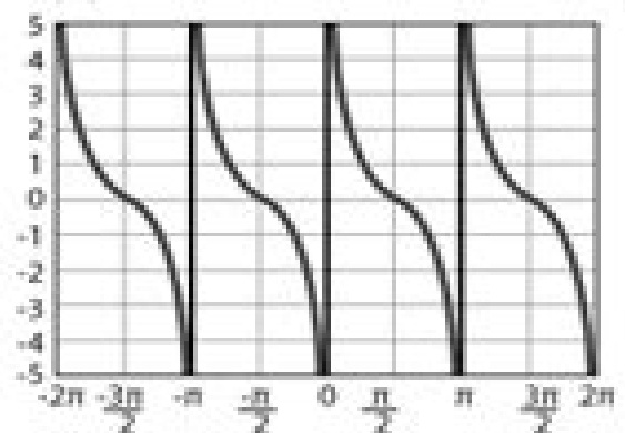
\cot(x)
