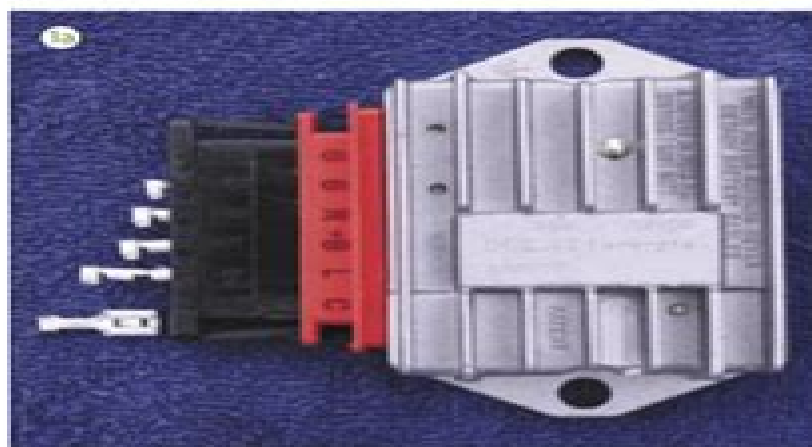
This Ducati rectifier-regulator is used to convert alternating current (AC) from the 912's internal generator to 12-volt direct current (DC) to power electronic accessories and charge the aircraft battery.
