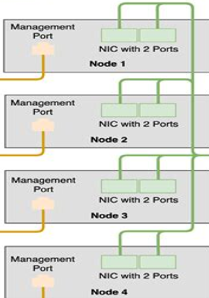
Out-of-Band Management Switch
