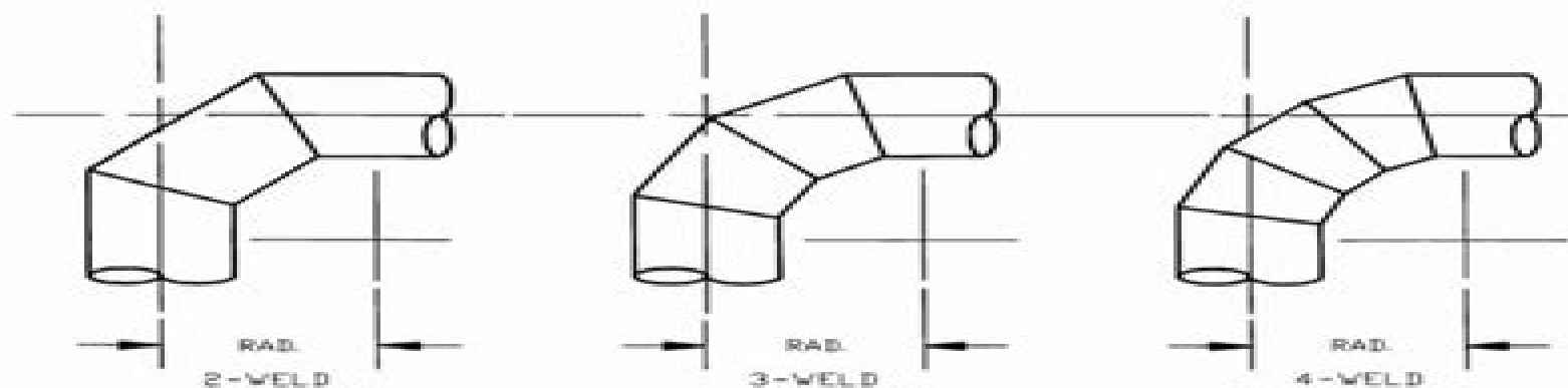
Figure 3-11. Mitered elbows.
