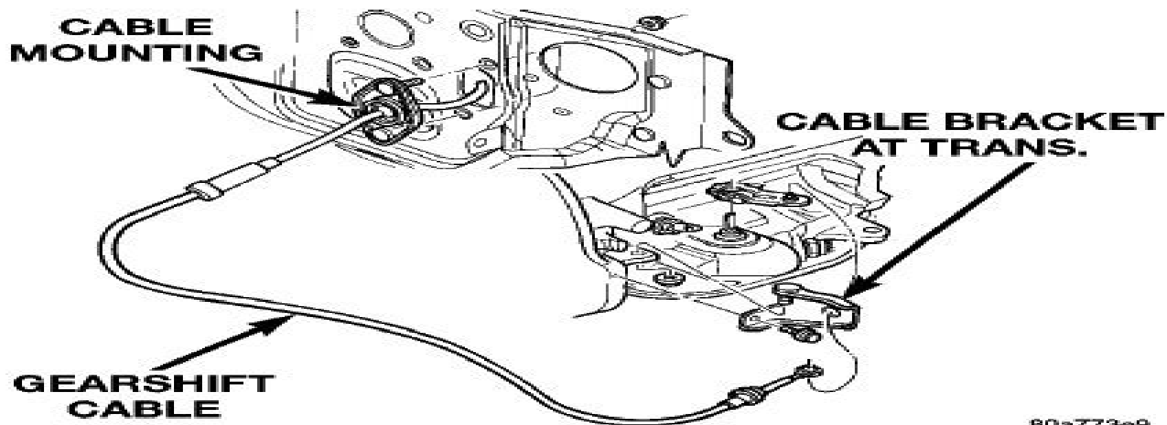
Fig. 249 Gearshift Cable Routing
