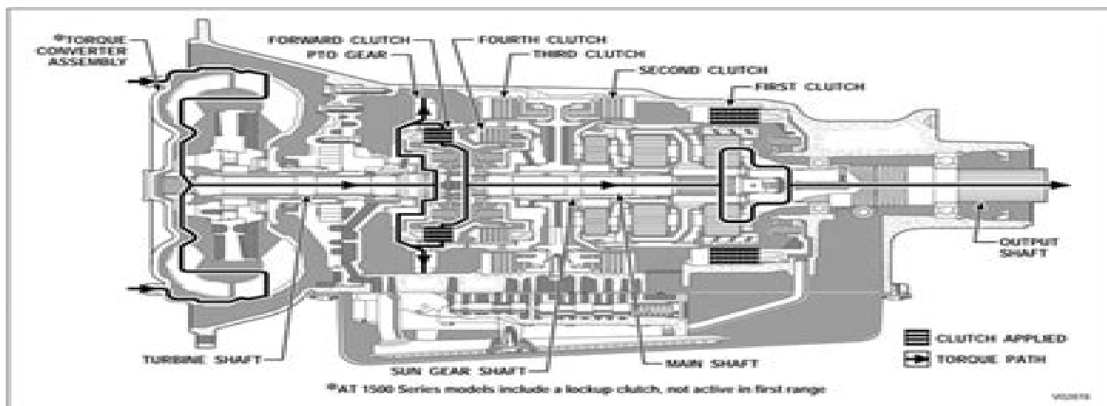
Figure 2-2. First Range Power Flow
