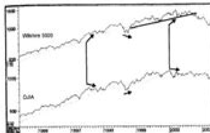
Chart 18-3 DJIA versus the Wilshire 5000, 1995–2001, and divergences. (From www.pring.com .)
