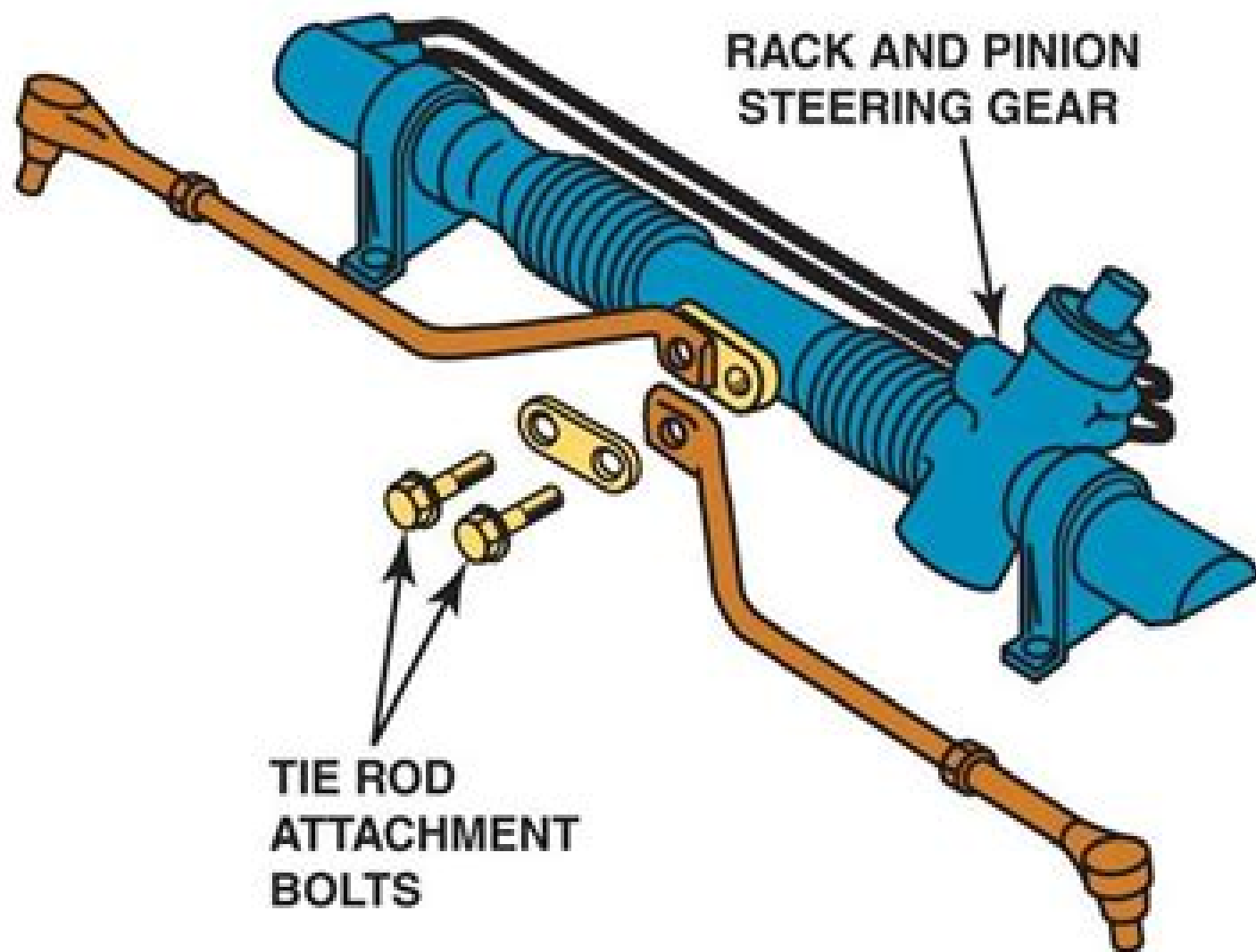
Figure 117-8 Exploded view of a center-take-off-style rack-and-pinion steering gear assembly.
