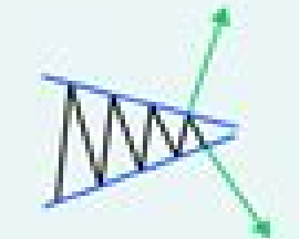
Symmetrical Triangle
