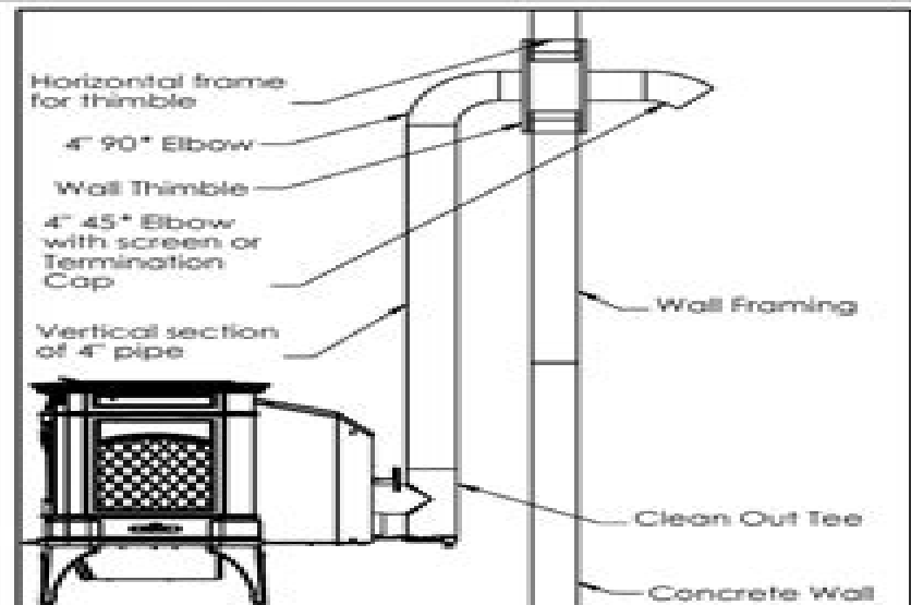
Figure 14: Venting with concrete wall behind unit.
