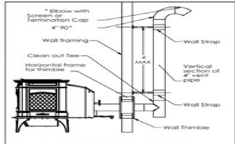
Figure 13: Venting horizontally with rise.
