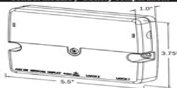
Control module / battery compartment
