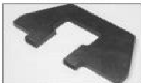
10.11a. The BMW tool for holding the camshaft in the TDC position on M40 engines.
