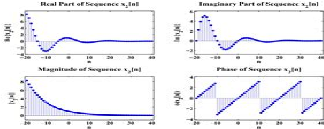
FIGURE 2.4: complex exponential signal x_2[n] = (0.9e^{j\pi/10})^n .
