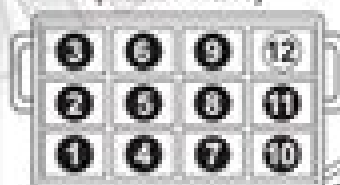
INPUT CONNECTOR (REAR VIEW)
