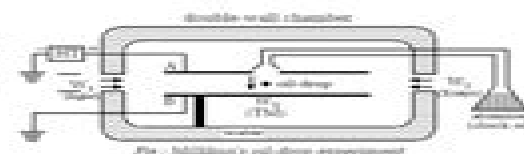
Fig. Millikan's oil drop experiment
