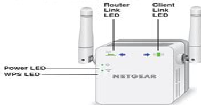
Figure 1. Extender front panel
