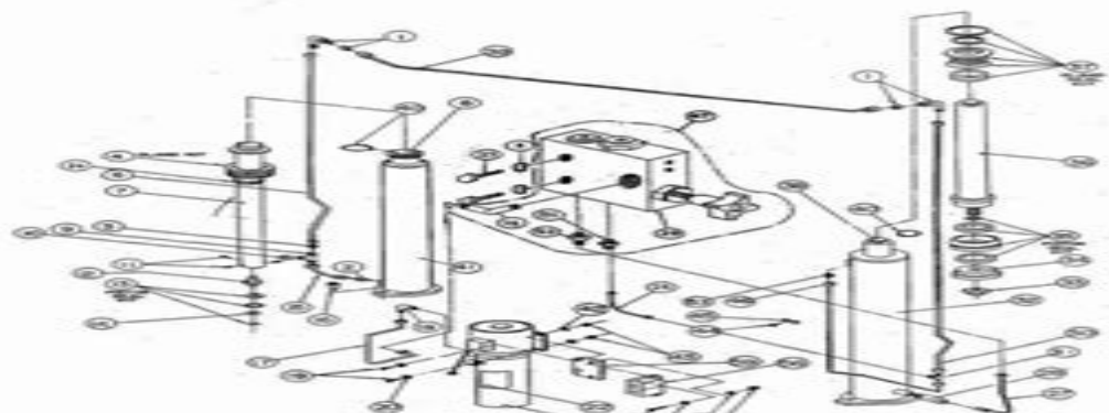
TWIN POST 8144 VECTOR HYDRAULIC PART LIST
