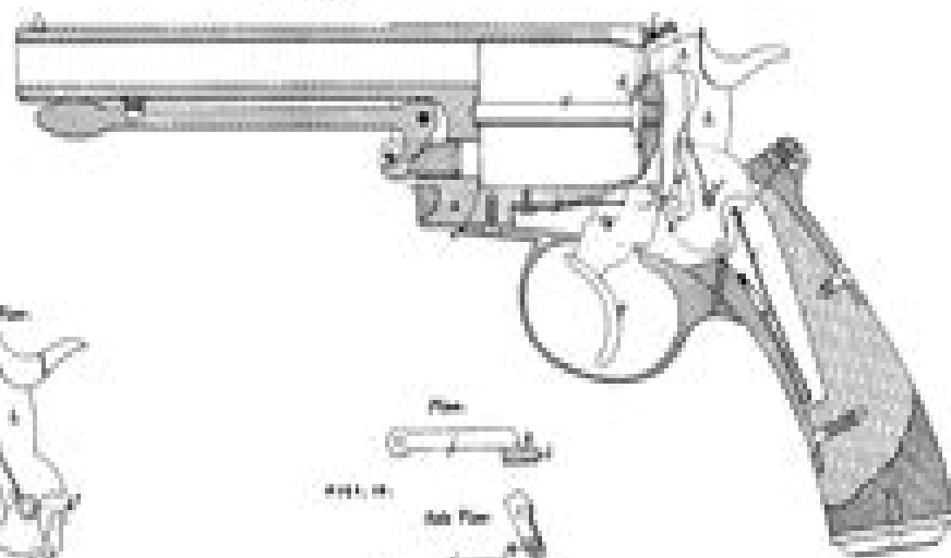
FIG. 3. Longitudinal Section.
