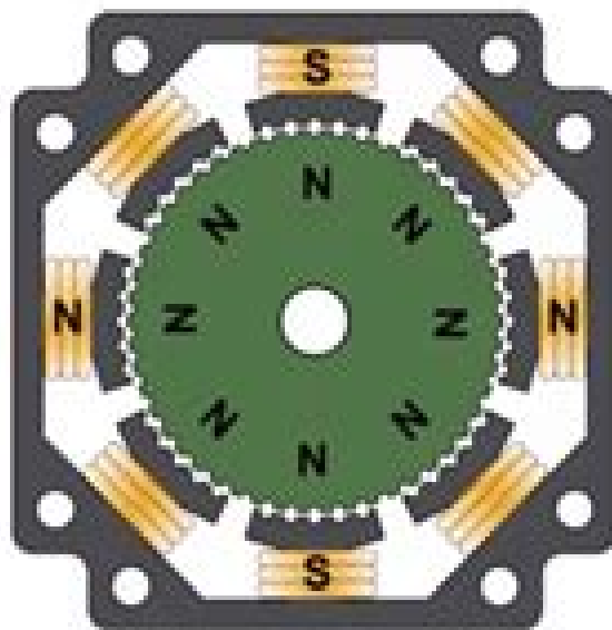
Step motor
