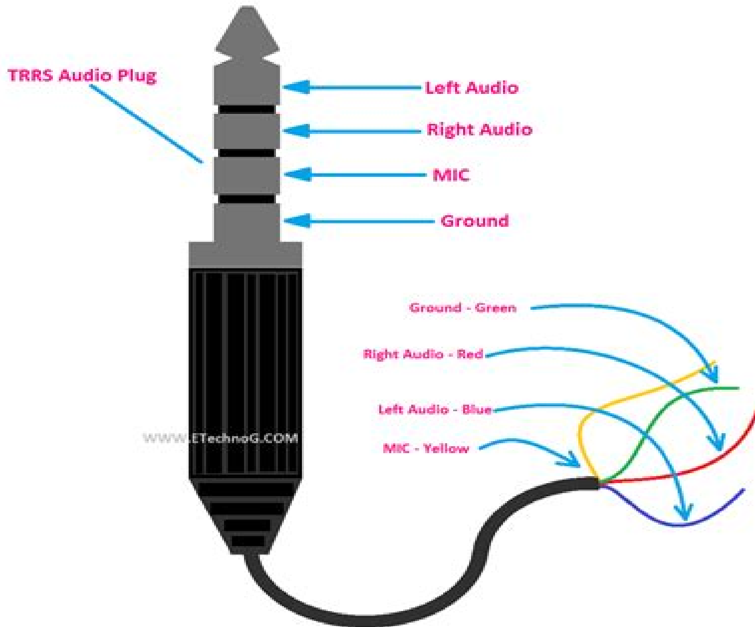
Headphone Jack Pinout and Color Codes
