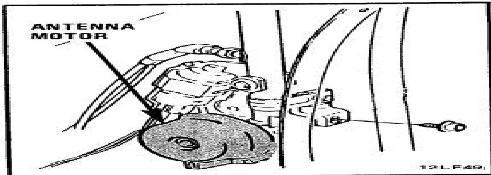
Figure E - In RH Front Fender
