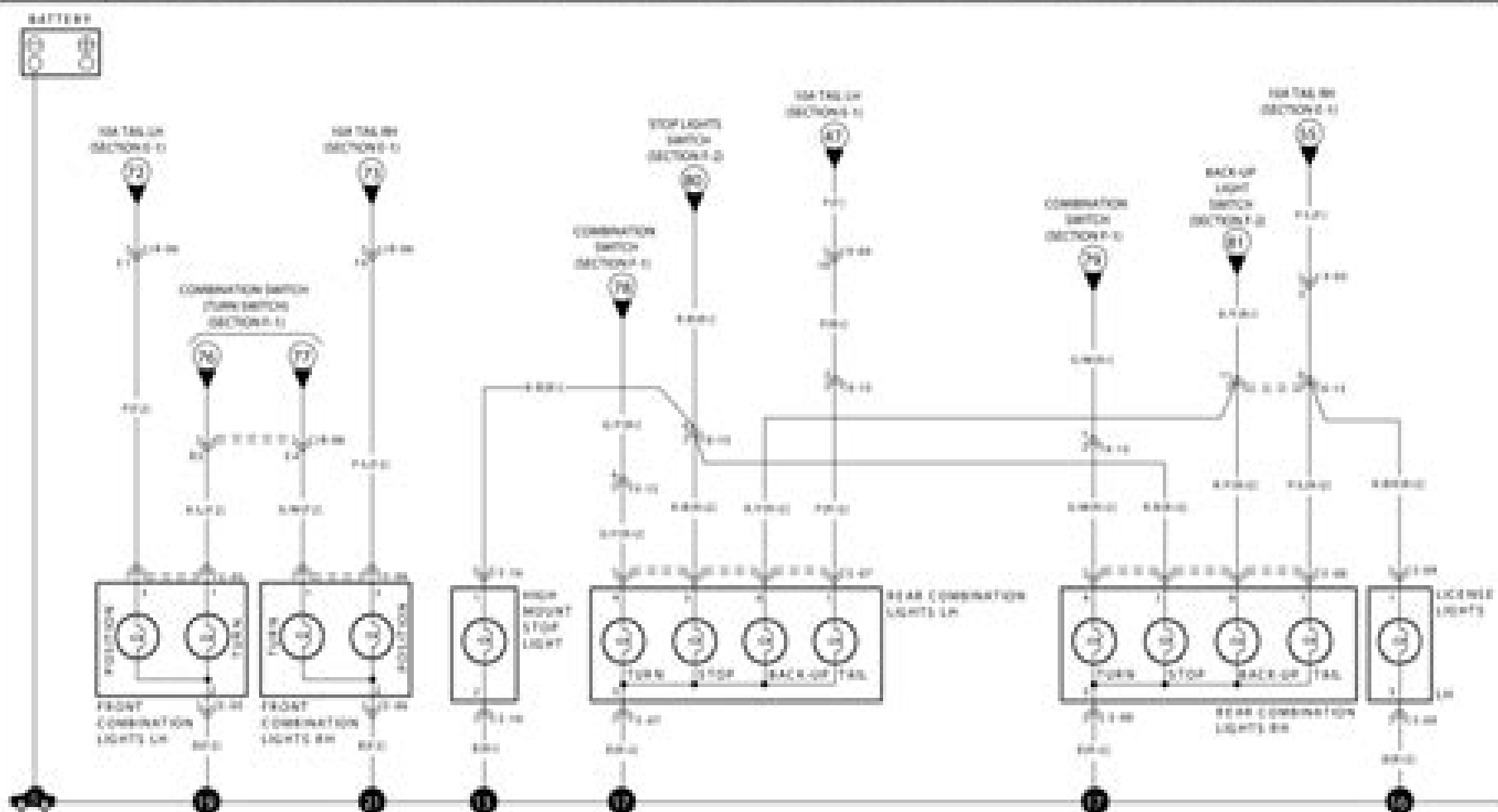
E-10 FRONT COMBINATION LIGHTS LH (P12-B)
