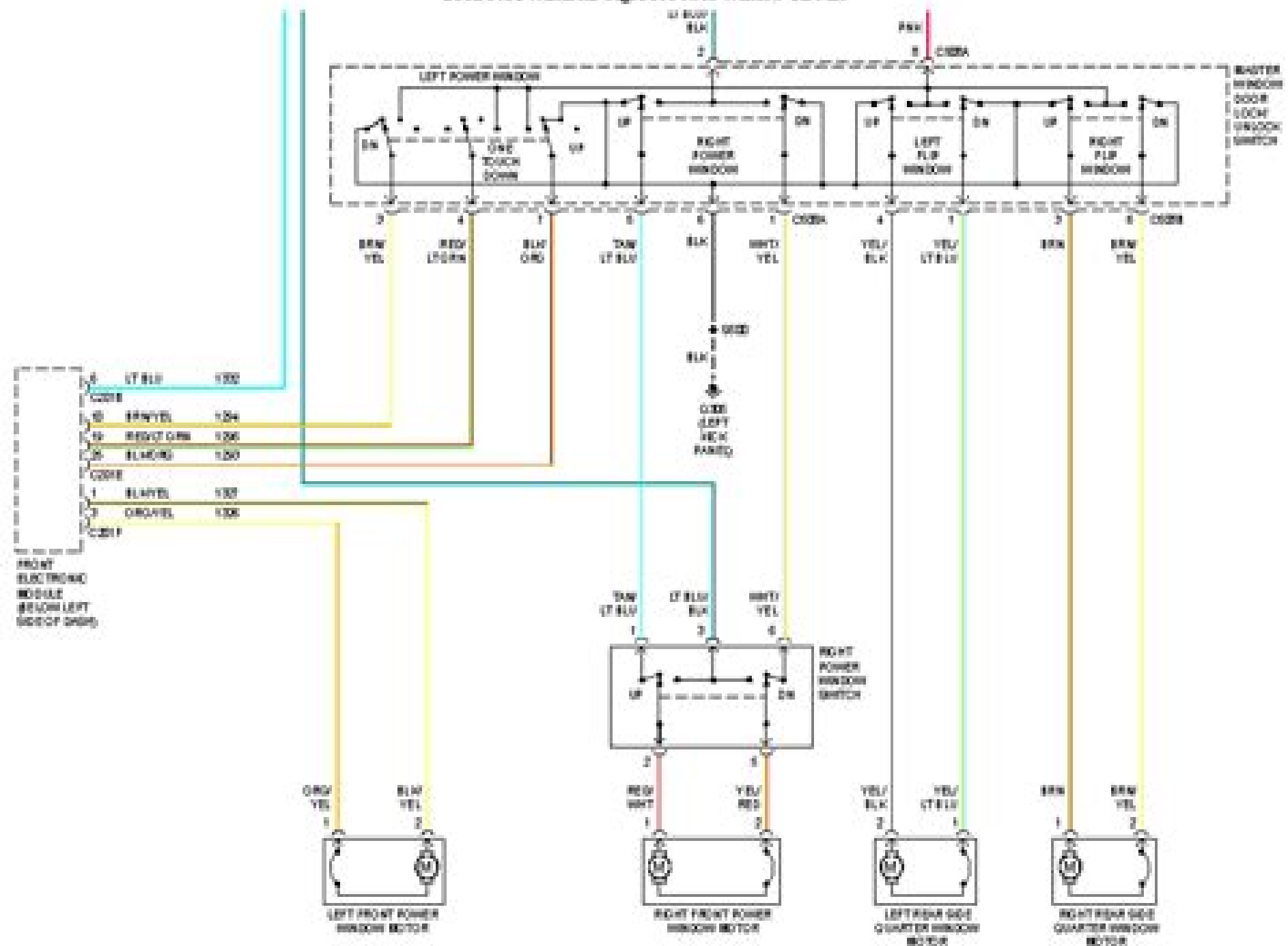
2002 Ford Windstar Fig. 50: Power Window Circuit
