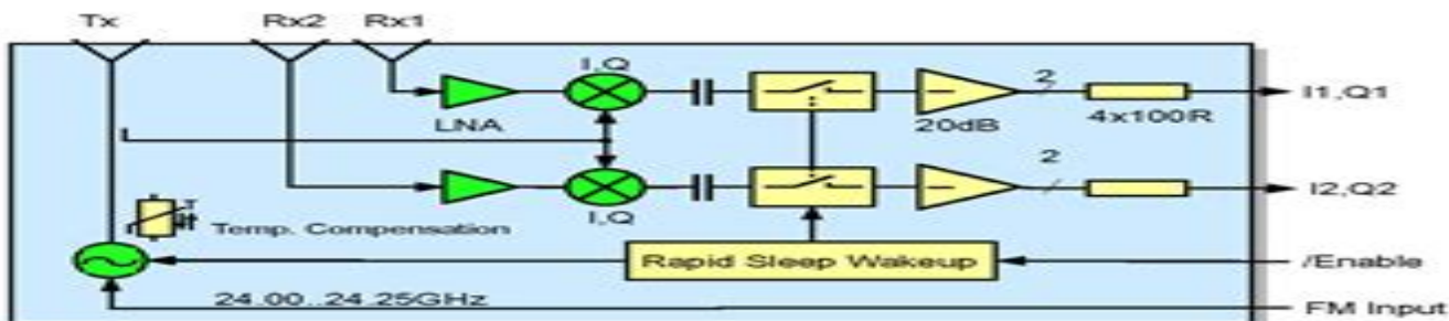
Fig. 1: K-MC4 Blockdiagram
