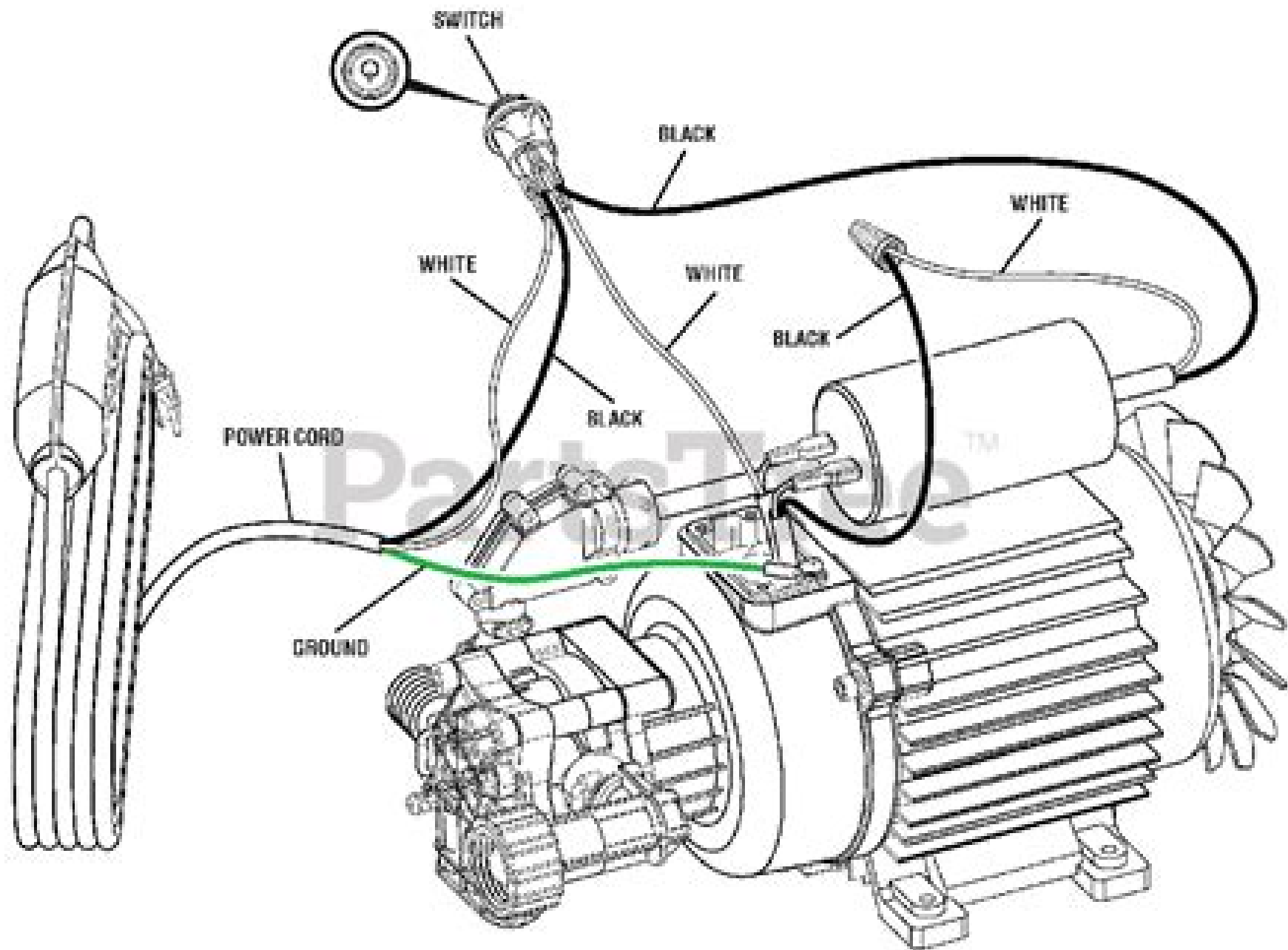
WIRING DIAGRAM
