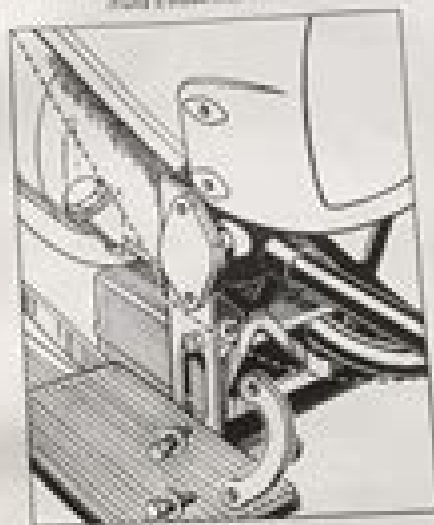
FIG. 14. REMOVAL OF BOLT FROM FRAME UNDER THE PLATE (Check to ensure that clear)
