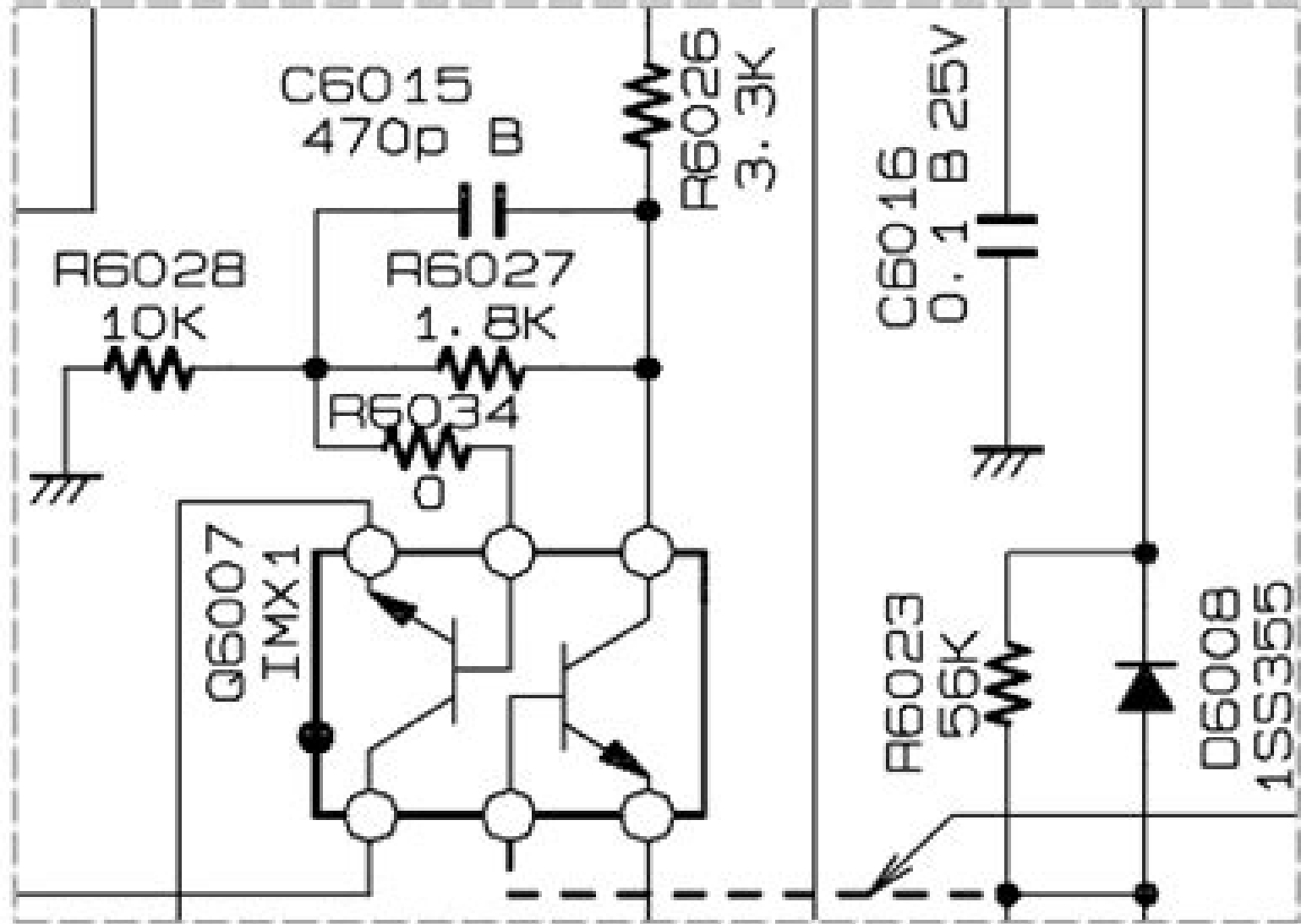
Preview: YAESU VXR-7000 schematic diagram
