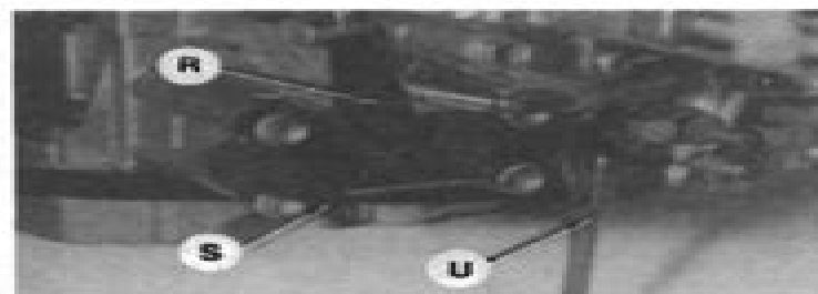
Fig. S218-23—Crankcase screw tightening sequence. Tighten 8 mm screws to 8-12 N·m (6-8 ft.-lbs.), 6 mm screws to 20-26 N·m (15-19 ft.-lbs.) and 10 mm screws to 46-54 N·m (34-39 ft.-lbs.).
