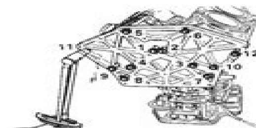
Fig. S218-24—To properly align cylinders to crankcase, install Suzuki cylinder/crankcase alignment tool 09912-68720, and tighten screws in sequence shown to 20-26 N·m (15-19 ft.-lbs.).
