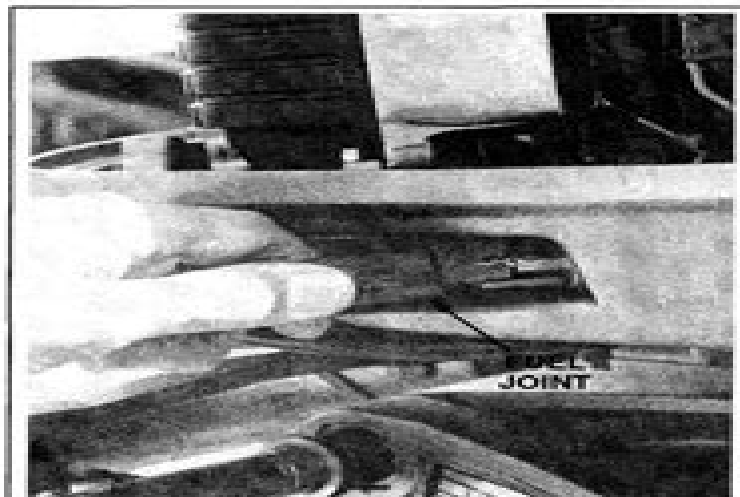
Fig. 84 Make a pre-season check of the fuel line coupling at the fuel joint to ensure a proper and clean connection
