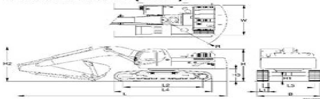
Figure 1 Dimensions of machine (EC360)
