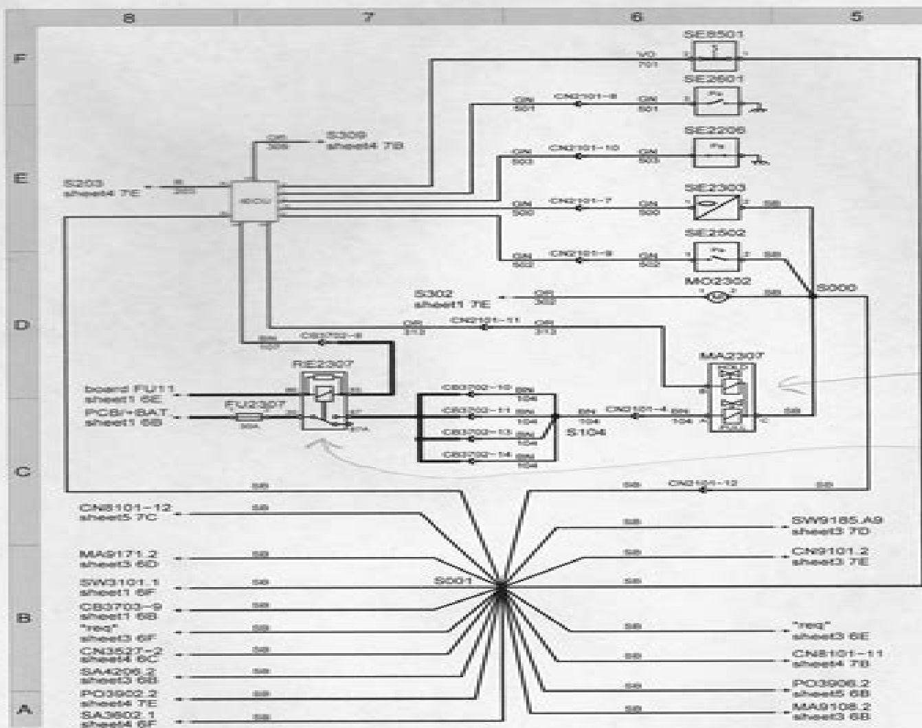
Figure 1 Wiring diagram 2
