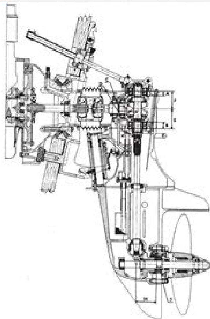
Fig. 40 Assembly drawing
