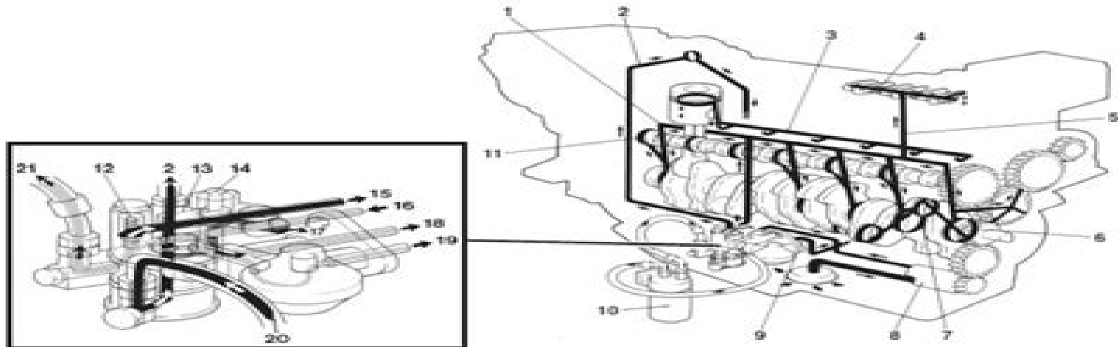
Lubrication system, TAMD 61, -62 and TAMD 71, -72.
