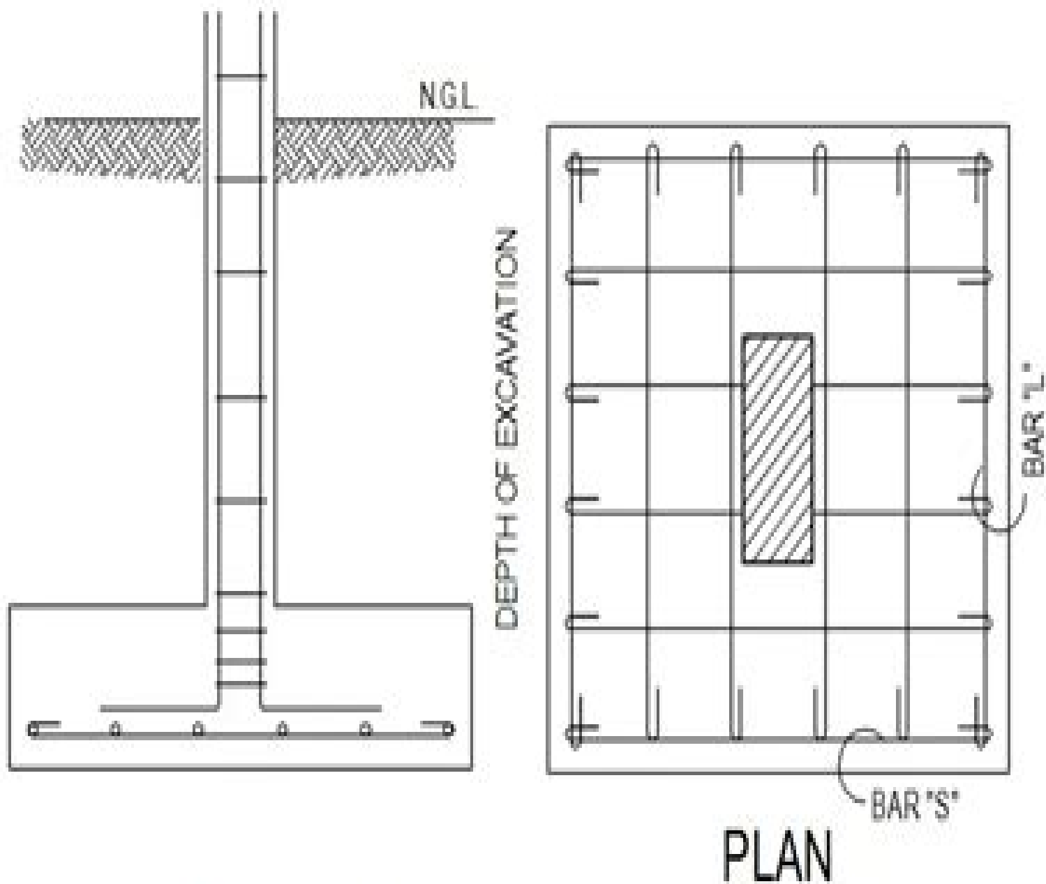
TYPICAL COLUMN/FOOTING DETAIL
