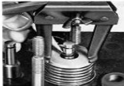
Fig. G.18. Locating a rubber 'O' Ring.
