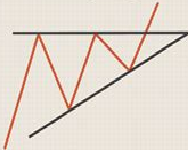
Ascending Triangle
