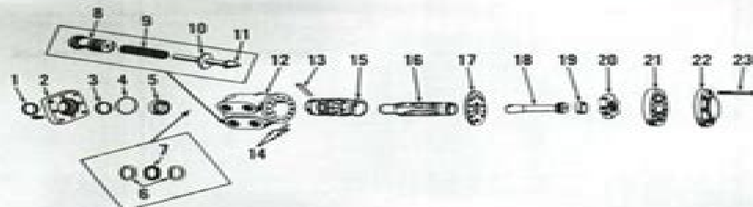
Fig. 8—Exploded view of steering control assembly. Centering springs (14) are installed in two rows of three springs with arch in each row back-to-back.
