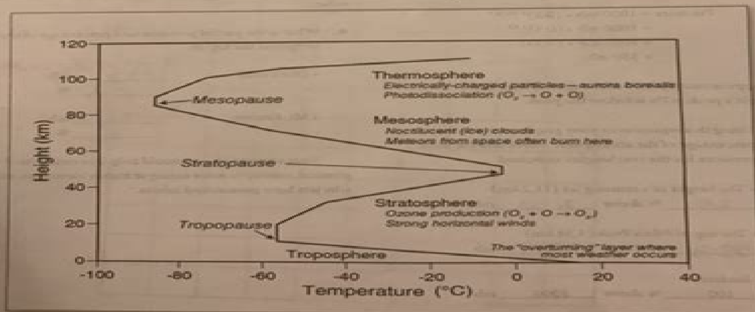
Figure 1-2. Layers of the atmosphere.
