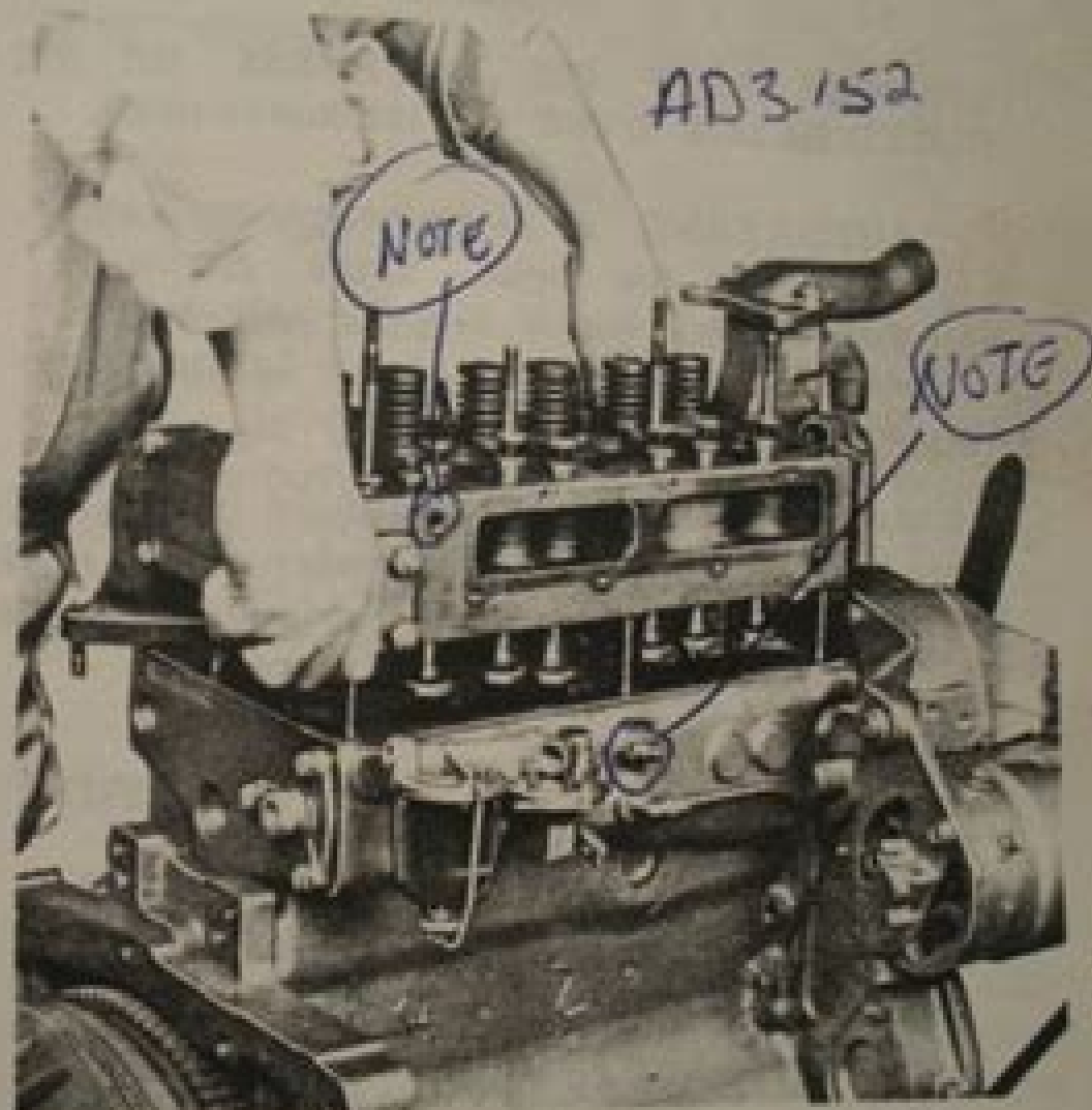
Fig. 9 - Removing or Installing the Cylinder Head
